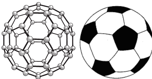
Figure 5: C_{60} molecule model and soccer ball
