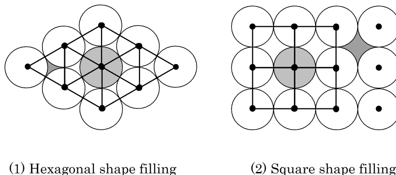
Figure 6: High density filling by circles
